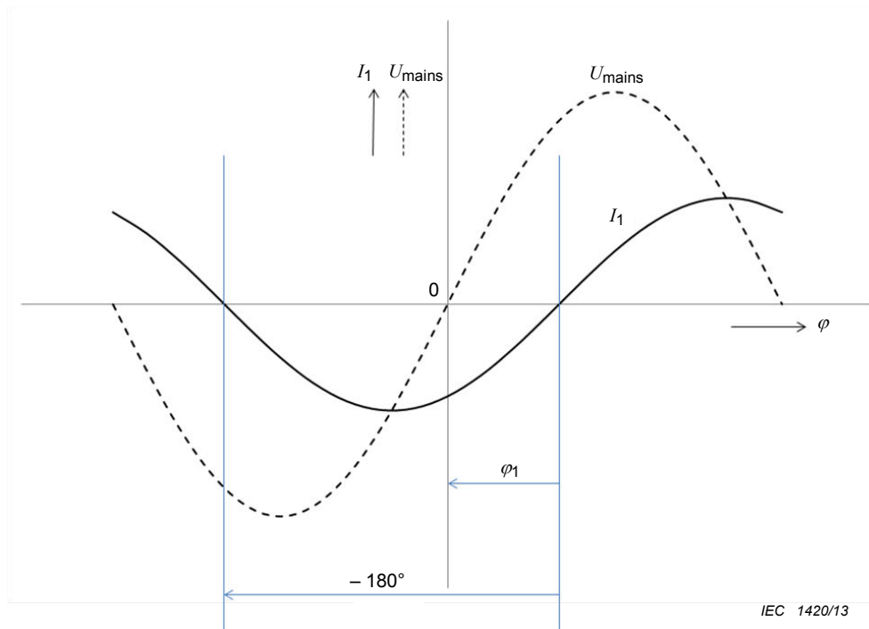
Figure C.2 – Definition of the 1 st harmonic current phase-angle ( \phi_1 ) ( I_1 lags U_{\text{mains}} , \phi_1 < 0 )
